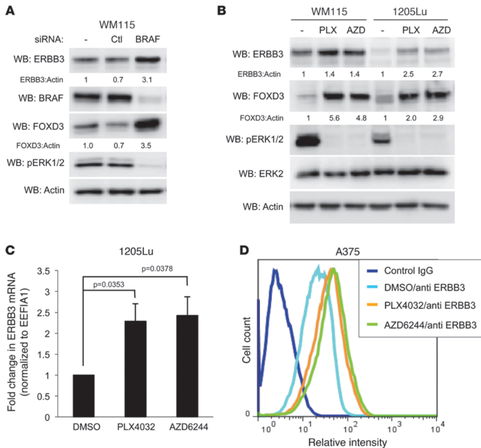
Figure 3 Inhibition of mutant BRAF and MEK1/2 enhances ERBB3 expression in melanoma cells. (A) WM115 cells were transfected with reagent alone (-), a nontargeting control siRNA (Ctl), or BRAF-targeting siRNA alone (BRAF) for 96 hours. Cells were lysed and immunoblotted as indicated. (B) WM115 and 1205Lu cells were treated overnight with DMSO (-), 1 μM PLX4032 (PLX), or 3.3 μM AZD6244 (AZD), lysed, and immunoblotted as indicated. (C) qRT-PCR analysis of ERBB3 mRNA levels in 1205Lu cells treated with DMSO, PLX4032, or AZD6244 overnight. Housekeeping gene EEF1A1 transcript was used for normalization. Results represent mean ± SEM (n = 4). P values are indicated. (D) Flow cytometry analysis of ERBB3 surface expression in A375 cells treated with DMSO, PLX4032, or AZD6244 overnight.
